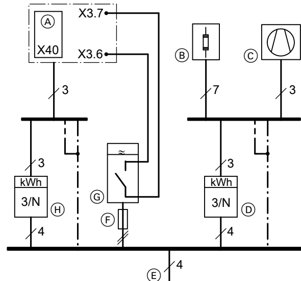
Fig. 36 Diagram excluding fuses and RCD
