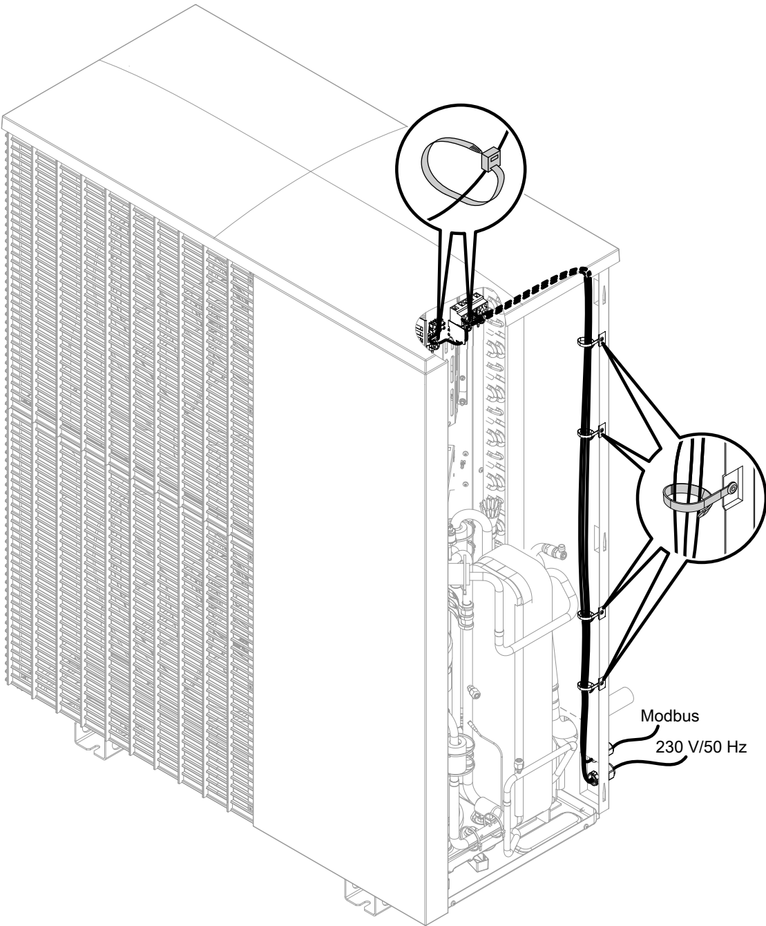
Fig. 41 Example: Type AWO-M-E-AC 201.A10
