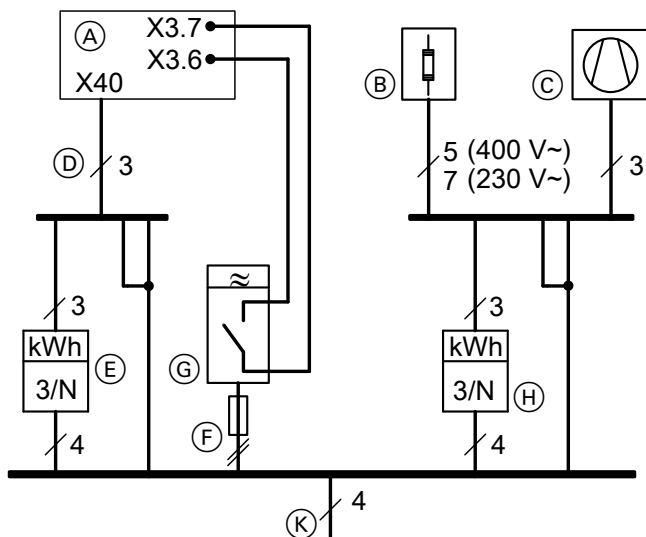
Fig. 51 Diagram excluding fuses and RCD
